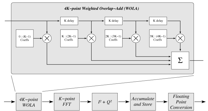
Fig. 5 Block diagram of the polyphase signal processing pipeline.
