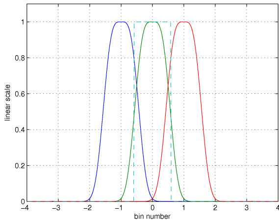
Fig. 6 Frequency response of the optimized FFT signal processing pipeline. The diagram shows three adjacent frequency bins. The dashed lines illustrate the equivalent noise bandwidth for the corresponding spectral bin.
