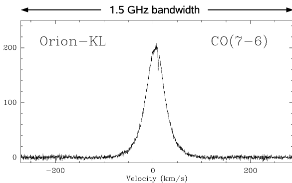
Fig. 4 First light spectrum of the new MPIfR-based 1.5 GHz bandwidth FFTS board towards the hot core Orion-KL. The high-excitation CO(7-6) transition at 806 GHz was observed with the central pixel of the CHAMP + array at APEX (24. October 2007).
