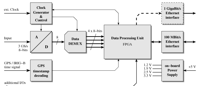
Fig. 2 Block diagram of the new MPIfR 1.5 GHz digitizer/analyzer board. The board can be equipped with a single- or dual-input ADC (ADC083000 or ADC08D1500). The optional GigaBit Ethernet interface allows high speed data acquisition with transfer rates up to 85 MBytes/s, which are required for pulsar or transient searches.
