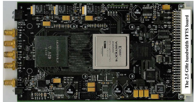
Fig. 7 Currently in development: The 2.5 GHz bandwidth FFTS. The board makes use of a first sample of E2V's 5 GS/s 8-bit ADC.
