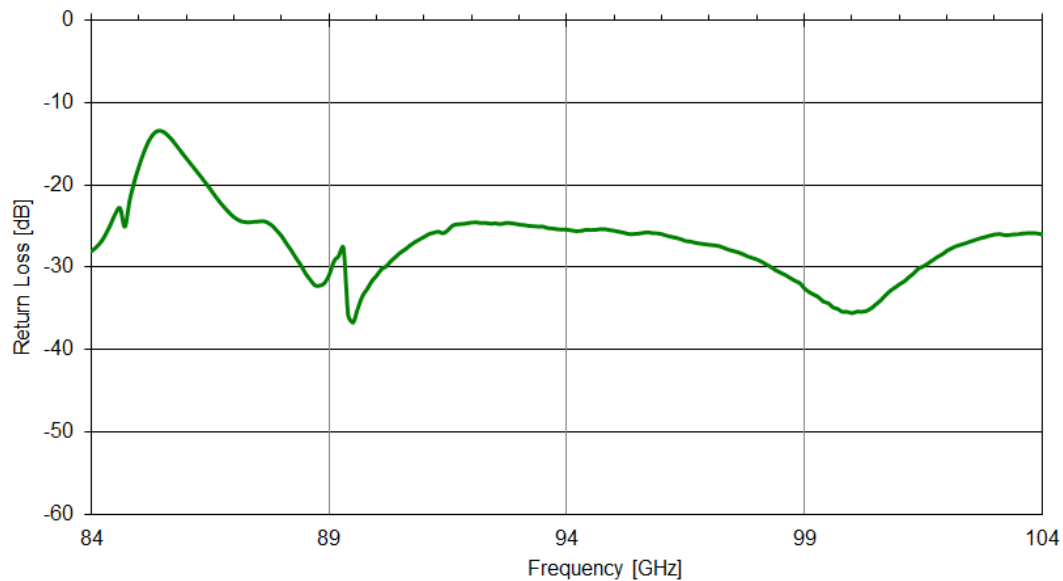
FH CG 94 - Return Loss
