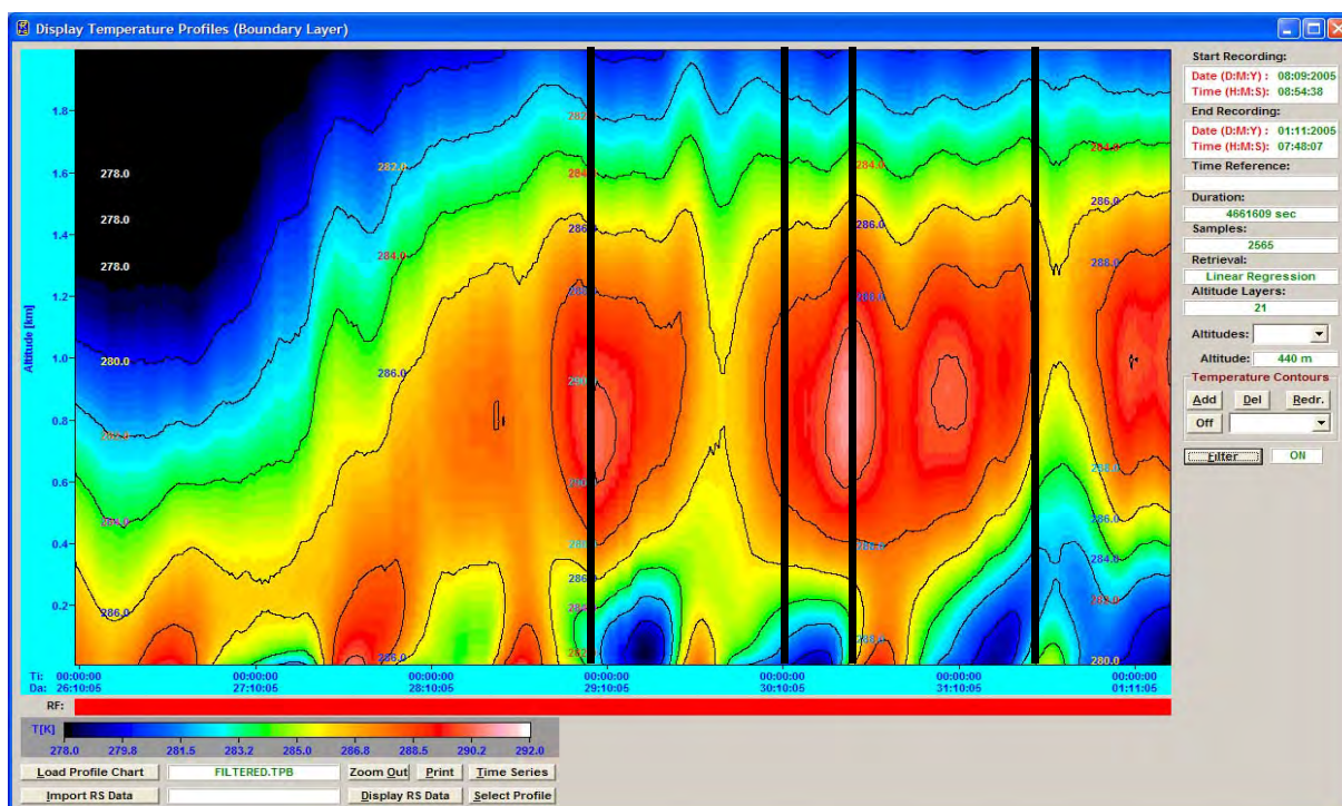
Fig.2.12: BLM map of one week period. Very strong inversions occurred in the second half of the period indicated by the black lines (Lindenberg, October 2005, courtesy of Univ.of Munich).
