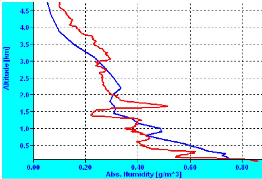
Fig.2.33: Humidity profile comparison from Pic du Midi (French Pyrenees), courtesy of CNRS, Laboratoire d'Aerologie, Observatoire Midi-Pyrenees.
