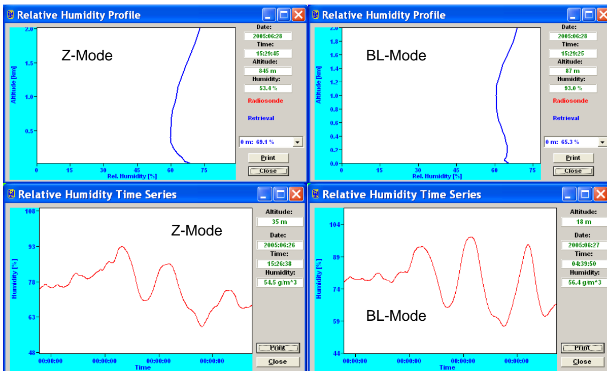
Fig:2.23: Relative humidity time series at low altitude measured in Z-mode and BL-mode. The BL-mode humidity maxima over night between 22:00 and 7:00 (when inversions are generated) are more pronounced than in Z-mode.
