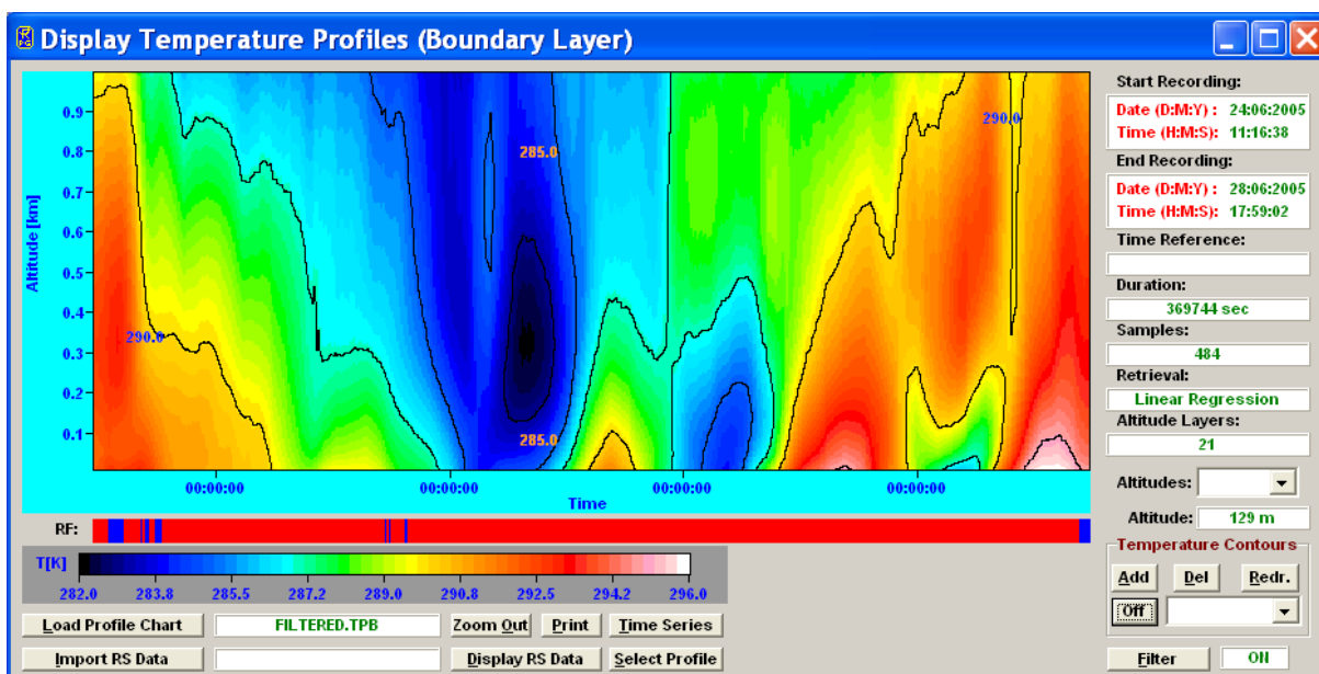
Fig.2.3b: Boundary layer scanning mode. The vertical structure even in the lowest layer <100 m is clearly resolved.
