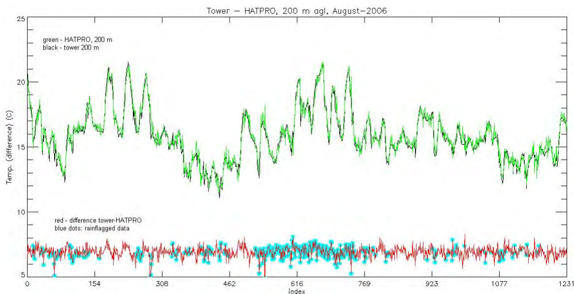
Fig.2.11: Comparison of retrieved HATPRO temperature at 200 m (green) with 200 m temperature sensor reading of met. tower (black) in Cabauw (KNMI) in August 2006. Total number of samples: 1232, no-rain: 836 samples (RMS: 0.36 K, bias: -0.04 K); 396
