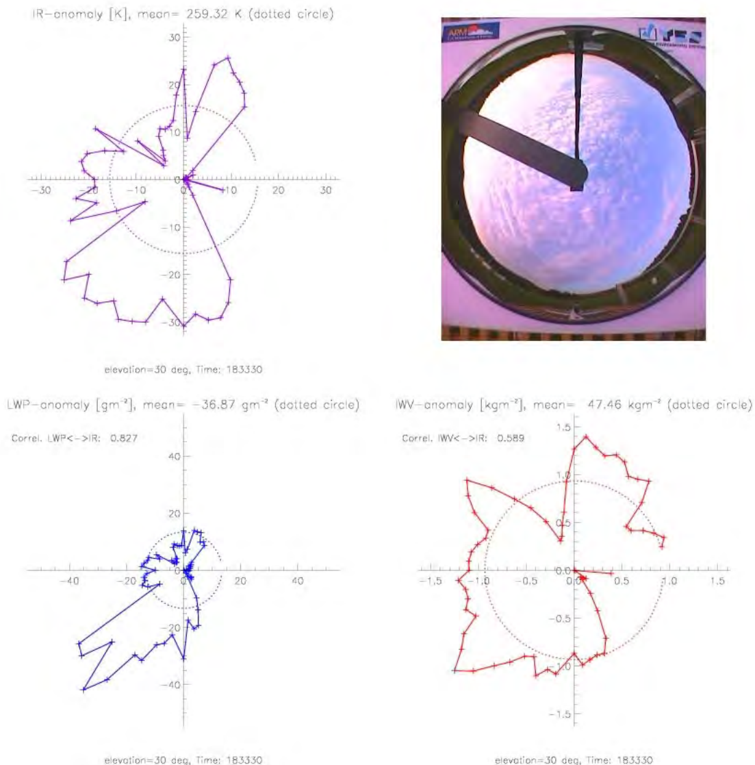
Fig.2.42: Under cloudy conditions, the IR radiometer signal is partially saturated while the microwave IWV is still reflecting the water vapour distribution. The IR gets saturated where the LWP level indicates clouds. Courtesy of S. Kneifel, Univ. of Cologne and LMU Munich.
