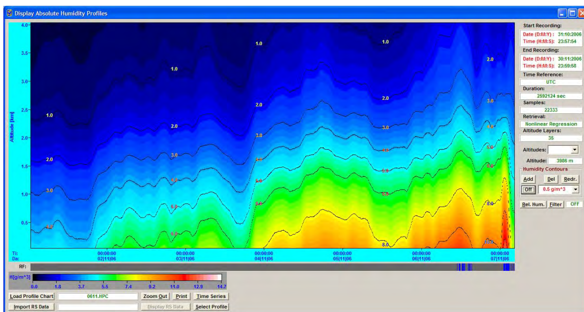
Fig.2.28: Absolute humidity profile map of the lowest 4000 m over 6 days.
