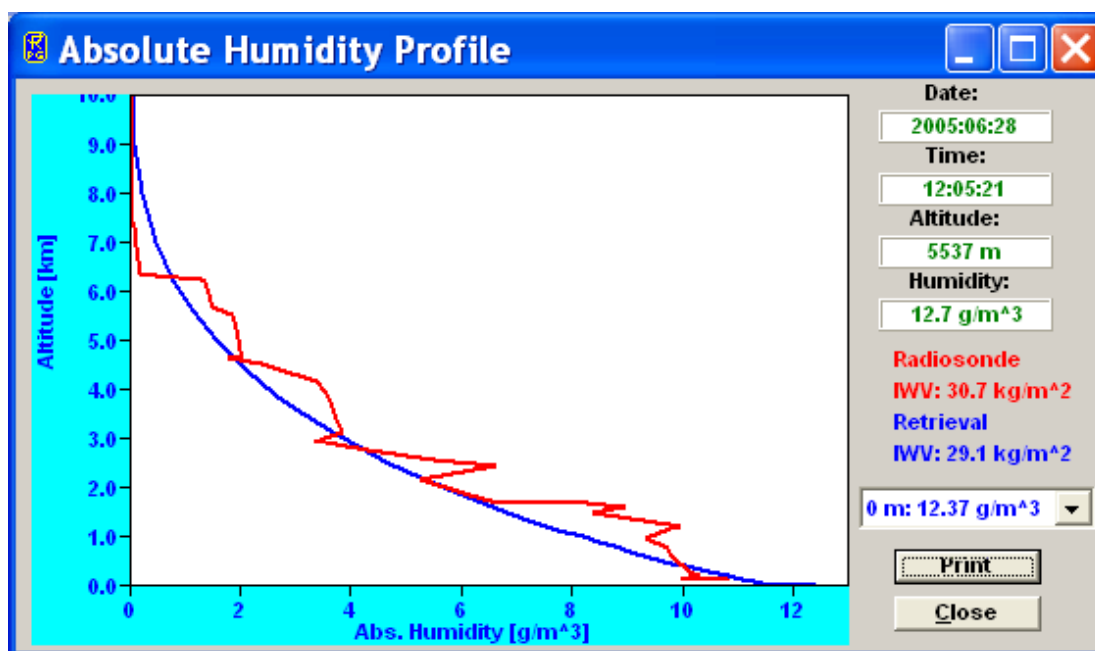
Fig.2.17: Sample profile taken from the map in Fig.16 at 12:00 UTC (noon time). In red is the data of a radiosonde for comparison (Larkhill, UK).
