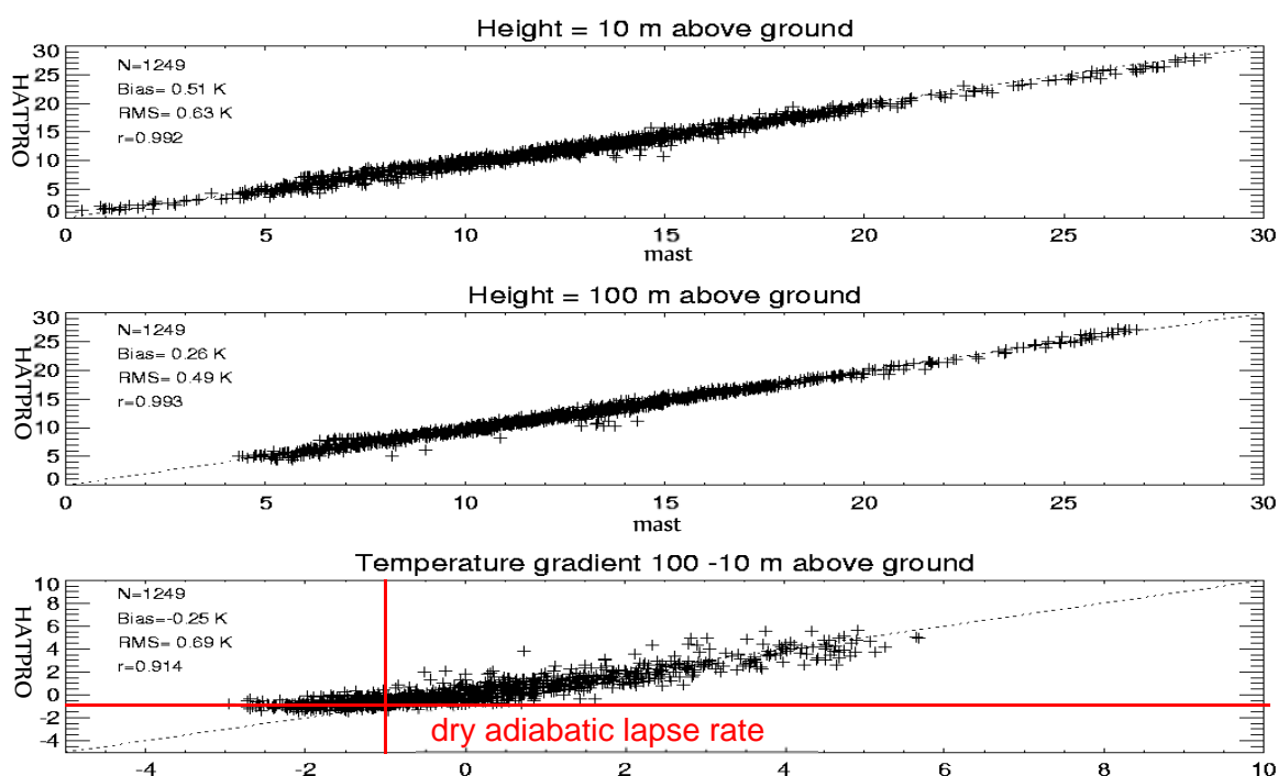
Fig.2.8c: Scatter plots of the comparison.
