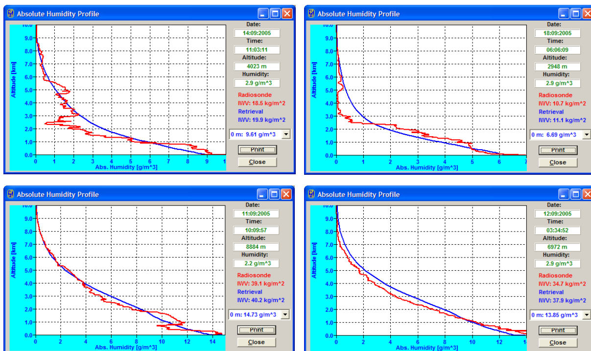
Fig:2.24: Absolute humidity profiles compared to radio soundings (red). Statistical analysis leads to RMS errors of 1 g/m 3 .
