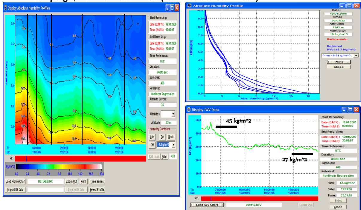
Fig.2.26: Example of a transition from wet to dry period by sea breeze effect in Benin / West Africa with development of absolute humidity profiles and integrated water vapour.
