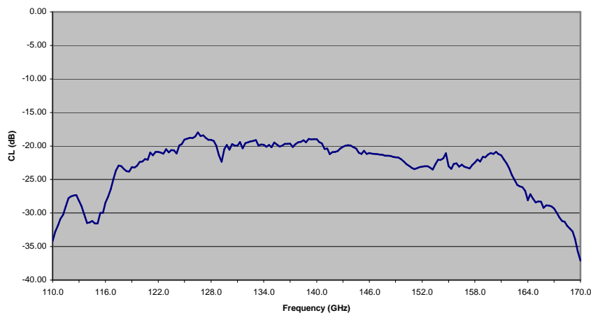
SAM-170 Conversion Loss
