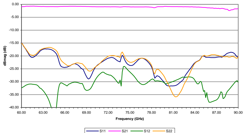
WFI-90 SN10054 S-Parameter
