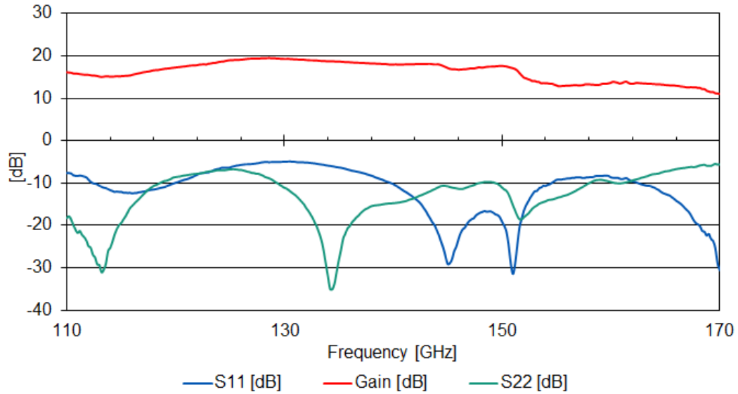
D-LNA 110-170 15-6 - Gain and Return Loss Performance
