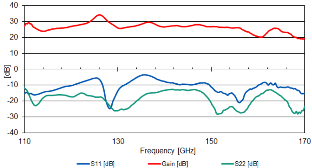
D-LNA 110-170 30 6 - Gain and Return Loss Performance
