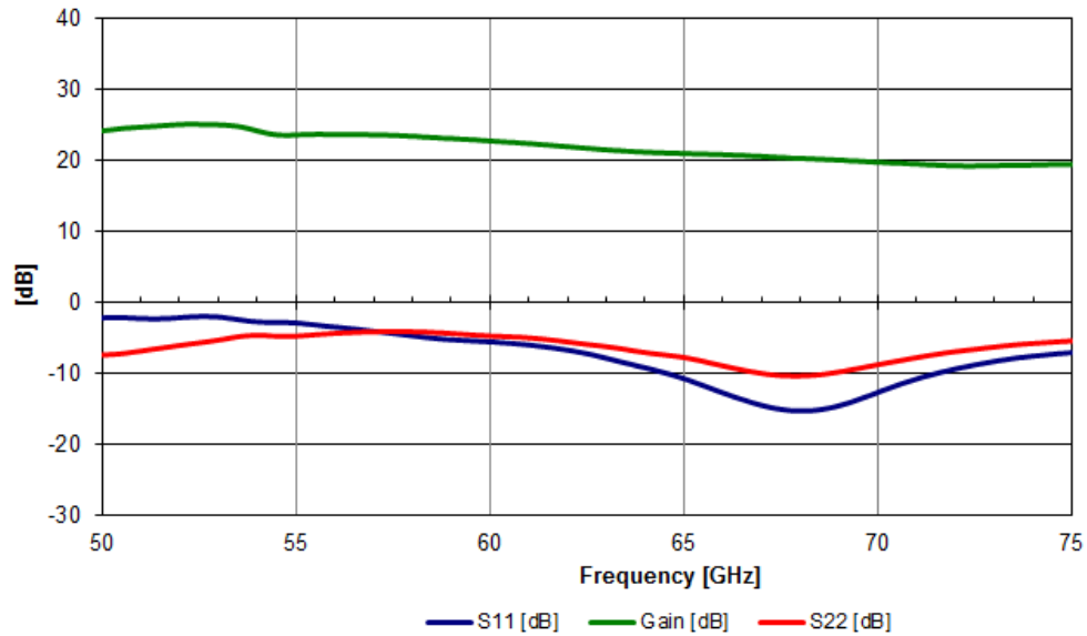
V-LNA 50-75 20 5 - Gain and Return Loss Performance
