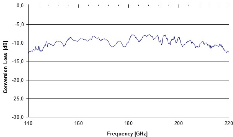
SHM-220 Conversion Loss
